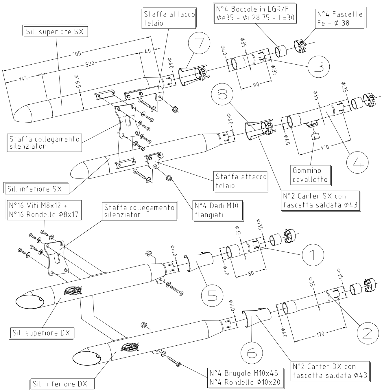
ART. 2258 YAMAHA XVZ 1300 ROYAL STAR Silvertail <<K02>> OMOLOGATO
