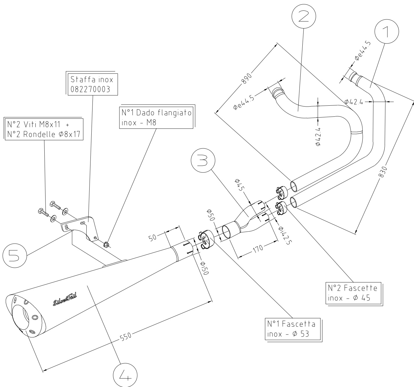
ART.2270 HONDA VT 750 BLACK WIDOW Silvertail <<PRO-S>> OMOLOGATO
