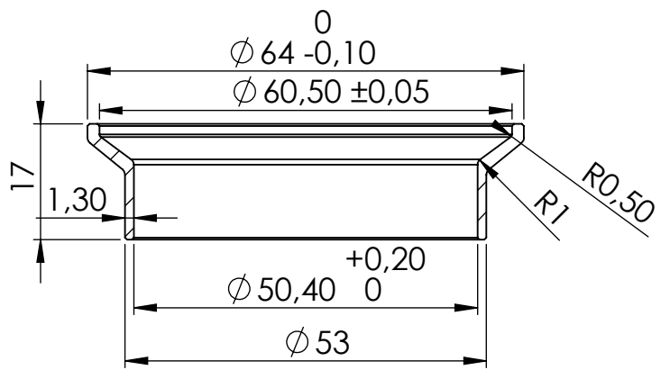
Bushing S.s. cod.206079
