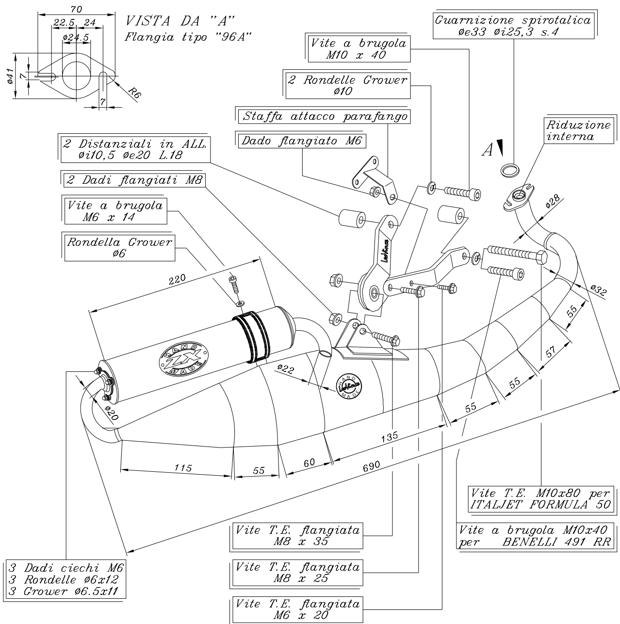
ART.4488 Silenziatore HAND MADE "ZX" per ITALJET FORMULA 50 (air cooled) BENELLI 491 RR '03 (liquid cooled)
